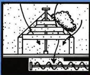
Stops chunks of grain that won't break up. Allows grain to flow around chunk.
