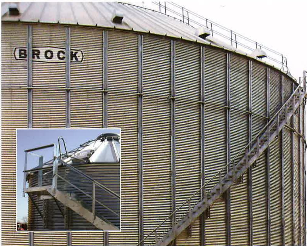
Stairway can be used with stiffened or unstiffened bins, or bins with wind rings.
